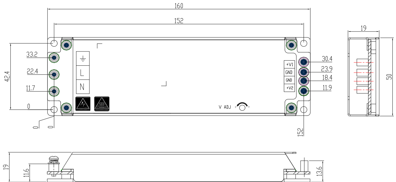
Dimensions and mounting holes - terminal coordinates
